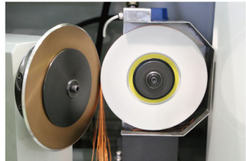
Grinding example of plane grinding wheel
